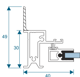
Slim-Line Equal Leg
