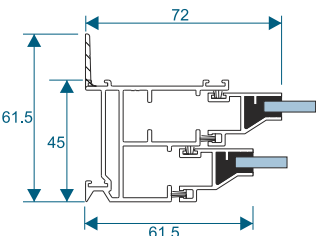
Slim-Line Equal Leg
