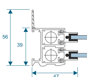
Slim-Line Equal Leg
