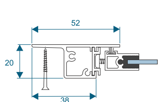
Economy Odd Leg
