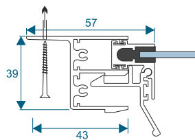
Economy Odd Leg
