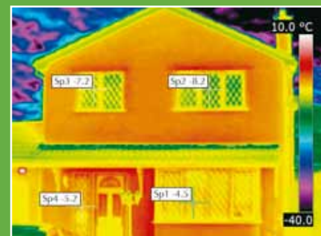
Red areas have been eliminated after fitting energy efficient VEKA windows.
